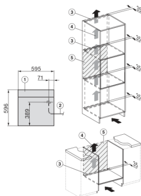
DGC7x60 connections and ventilation 60cm, installation drawing
