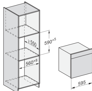
built-in DGC XXL, installation drawing
