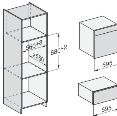
Installation DGC XXL, ESW7x20 installation drawings
