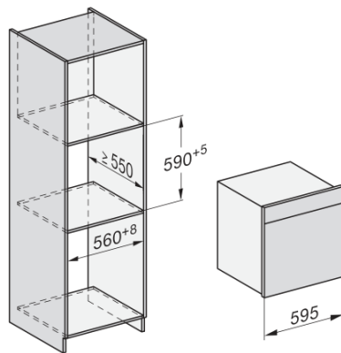
built-in DGC XXL, installation drawing
