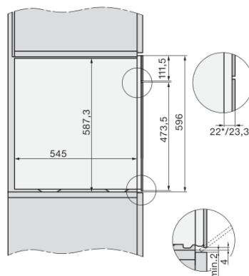
side view DGC XXL, installation drawings
