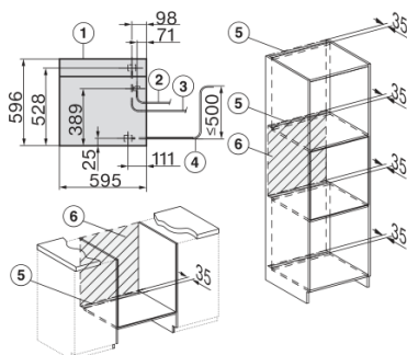
DGC7x65 connections and ventilation 60cm, installation drawing
