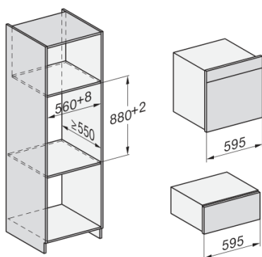
Installation DGC XXL, ESW7x20 installation drawings
