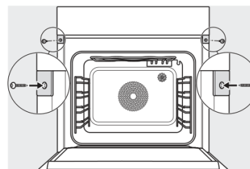
built-in DGC XXL, installation drawing
