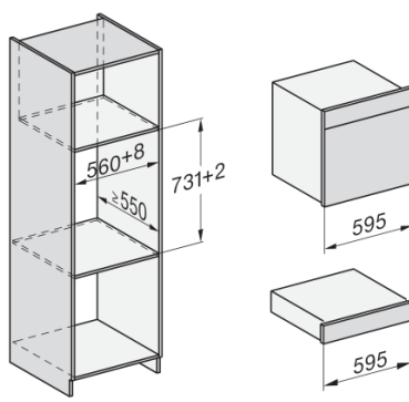
Installation_DGC_XXL_ESW7x10_EVS7010 installation drawings
