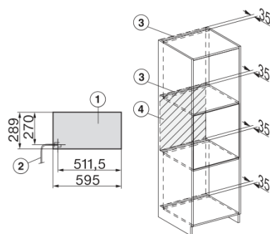
Installation, ESW7x20, DGM7x4x installation drawings
