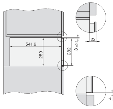
side view ESW7x20, installation drawing, GB, AU
