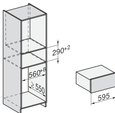
built-in ESW7x20, installation drawing
