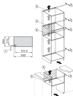
Installation ESW7x20, installation drawing, GB, AU
