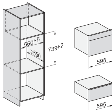
ESW7020, Installation drawings, XL combination niche height
