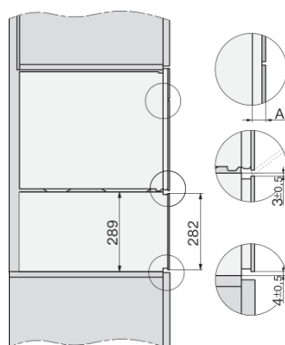
side view, DG, DGM, ESW7x20 installation drawings
