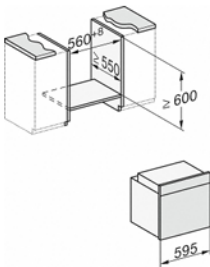
H226x-1B/BP/E/EP/MP, H2x6xB/BP, H7x6xB/BP/BPX, installation drawings
