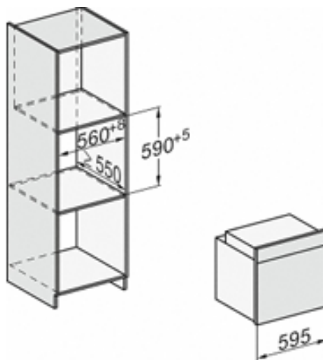
H226x-1B/BP/E/EP/MP, H2760B/BP, H28x0B/BP, H7x6xB/BP/BPX, installation drawings
