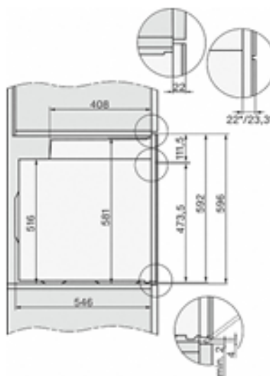
H2x6x-1B/BP/E/EP/MP, H2850BP, H7x6xB/BP/BPX, H2x6xB, installation drawings
