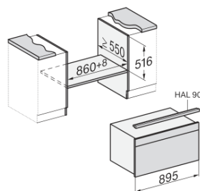
built-in H7000 90 built-under, installation drawing If the oven is to be installed under a hob, follow the instructions for installing the hob and the height of the hob.
