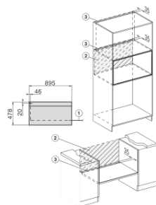
installation H7000 90, installation drawing 1) Mains connection cable, L=2000 mm, 2) No connection in this area, 3) Lüftungsausschnitt min. 150 cm²
