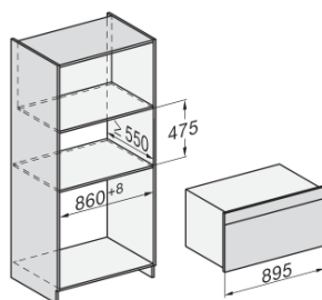
built-in H7000 90, installation drawing
