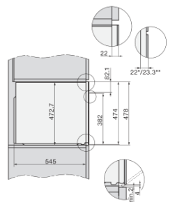
side view H7000 90 D1, installation drawings, GB, AU 22 mm – glass, 23.3 mm – metal
