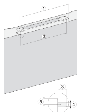
H7000 handle, installation drawing 1) 400 mm, 2) 360 mm, 3) 47 mm, 4) 24 mm, 5) 32.5 mm
