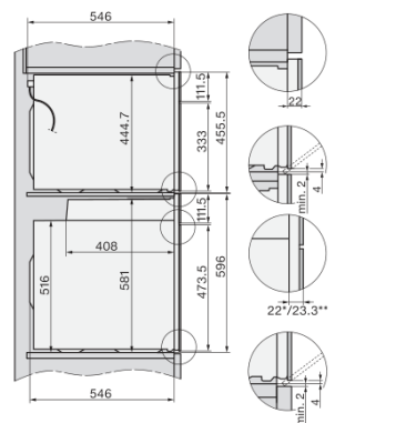
Side view Kombi BM XL, installation drawings 22 mm – glass, 23,3 mm – metal
