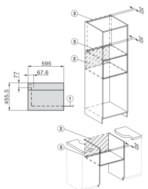
Installation H7000BM, installation drawings, GB, AUS 1) Mains connection cable, L=2000 mm, 2) No connection in this area, 3) Lüftungsausschnitt min. 150 cm 2
