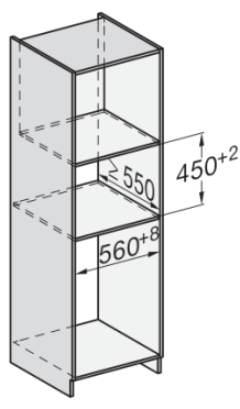
built-in H7000 BM, installation drawing
