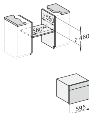
built-in H7000 BM build-under, installation drawings
