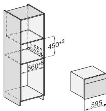
built-in H7000 BM, installation drawing
