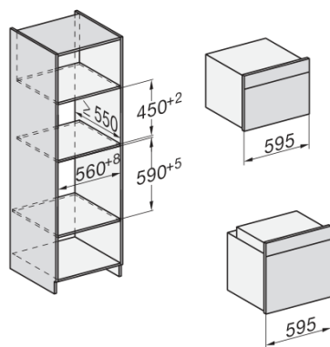
Installation H7000 BM XL, installation drawings
