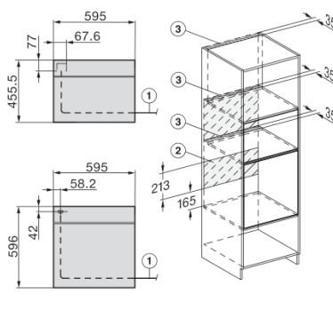
Installation Kombi BM XL, installation drawings
