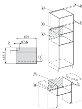
Installation H7000BM, installation drawings, GB, AUS
