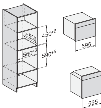
Installation H7000 BM XL, installation drawings
