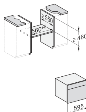
built-in H7000 BM build-under, installation drawings
