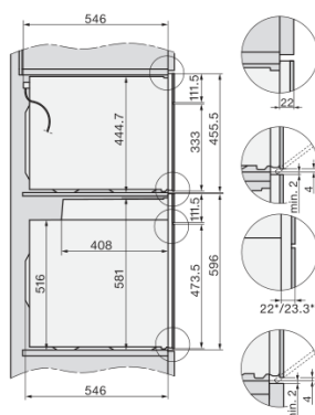
Side view Kombi BM XL, installation drawings
