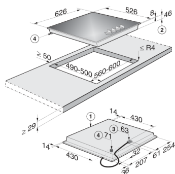
KM 3010 G (Installation drawing)
