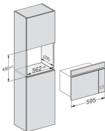
M223xSC, Skizze
