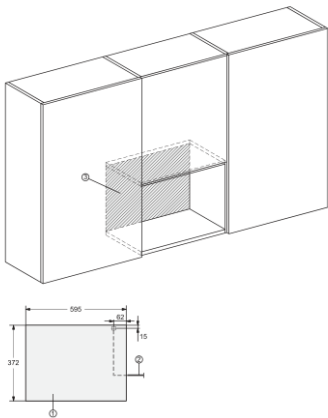
M2230SC, Skizze
