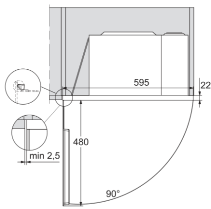
M223xSC, Skizze
