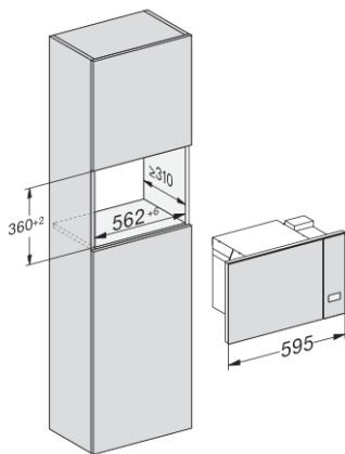
M223xSC, Skizze
