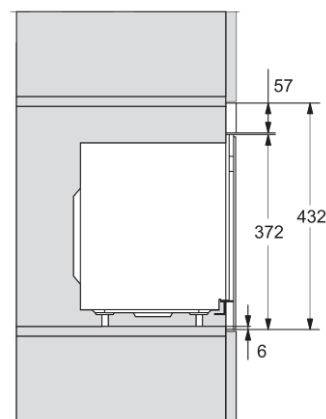
M223xSC, Skizze
