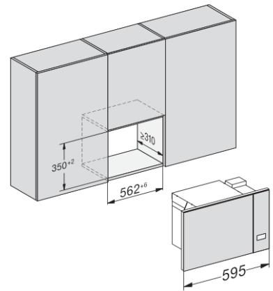
M223xSC, Skizze
