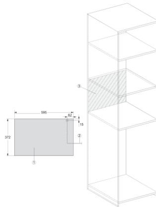
M223xSC, Skizze
