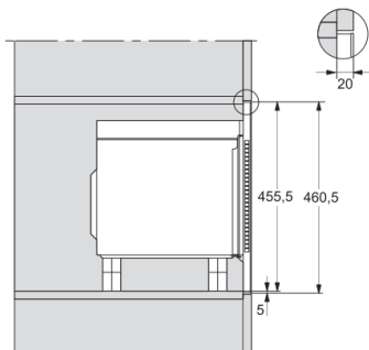
M2240SC, installation drawing
