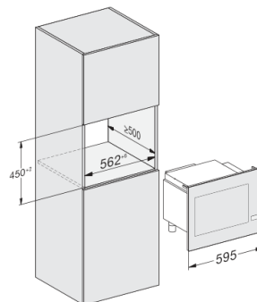
M2240SC, installation drawings
