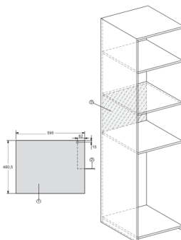
M2240SC, installation drawings
