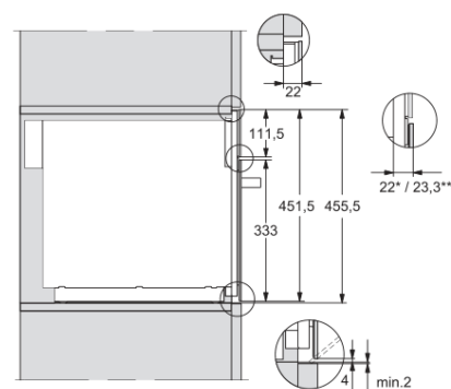
M7140TC, M724xTC, Skizze 22 mm – Glas, 23.3 mm – Edelstahl
