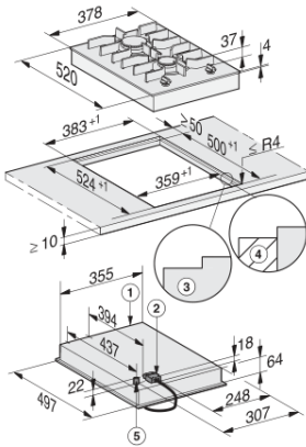
CS7102FL, CS7102-1FL flush (installation drawing)
