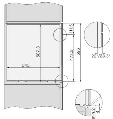
screw joint DGC XXL, installation drawing
