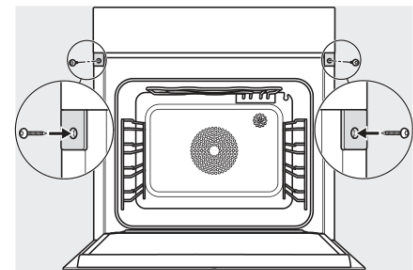
built-in DGC XXL, installation drawing
