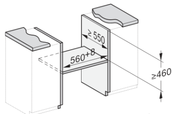
Installation_DG_DGM_DGC_XL_ESW7x10_EVS7010, installation drawings
