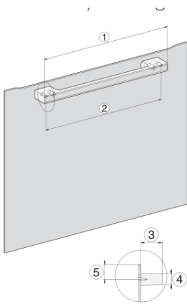
H7000 handle, glass, installation drawings
