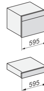
Installation_DG_DGM_DGC_XL_ESW7x10_EVS7010, installation drawings
