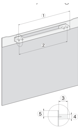
H7000 handle, installation drawing
