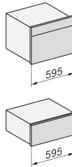
Installation DG, DGM, DGC XL, ESW7x20 installation drawings
