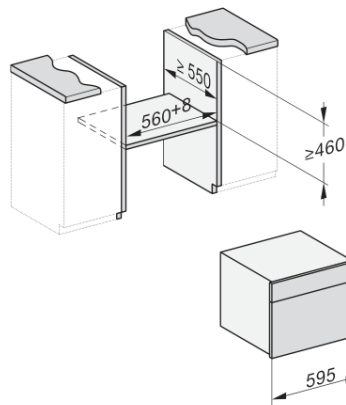
Installation_DG_DGM_DGC_XL_ESW7x10_EVS7010, installation drawings
