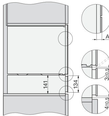
Side view_DG_DGM_ESW7x10_EVS7010 installation drawings
