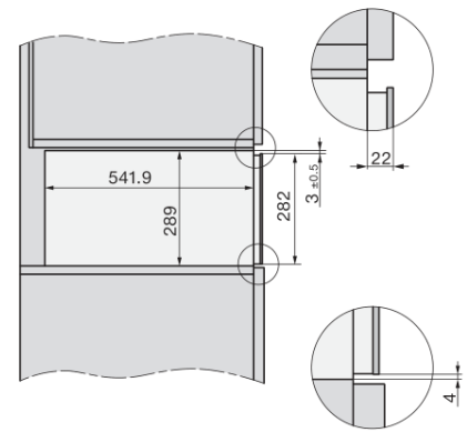
side view ESW7x20, installation drawing, GB, AU
