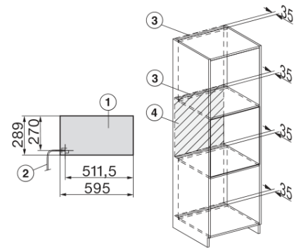
Installation, ESW7x20, DGM7x4x installation drawings
