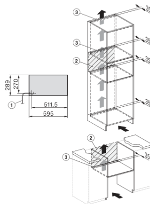
ESW7020, Installation drawings, XL combination niche height
