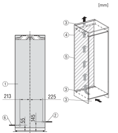
FNS7794D L, FNS7794D R, installation 1. View from the front. 2. Mains connection cable. L
