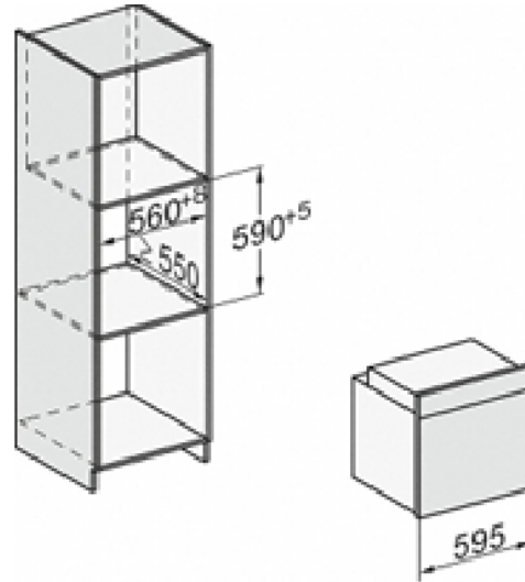
H226x-1B/BP/E/EP/VP, H2760B/BP, H28x0B/BP, H7x6xB/BP/BPX, installation drawings
