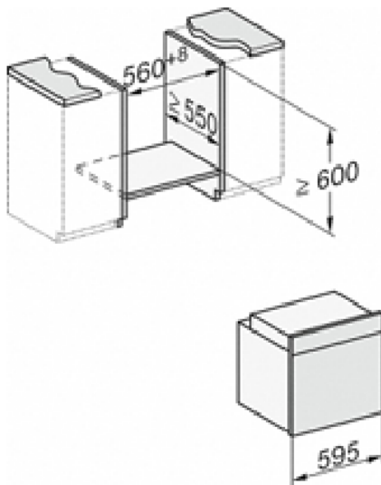
H226x-1B/BP/E/EP/VP, H2x6xB/BP, H7x6xB/BP/BPX, installation drawings
