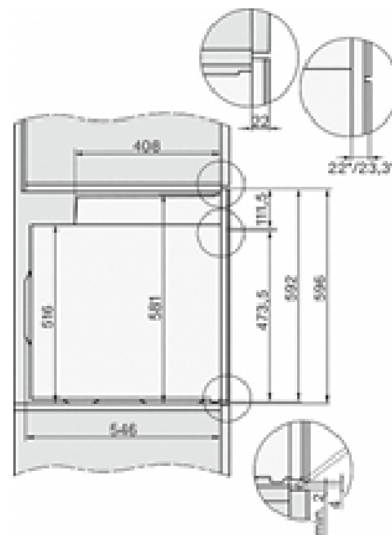
H2x6x-1B/BP/E/EP/VP, H2850BP, H7x6xB/BP/BPX, H2x6xB, installation drawings
