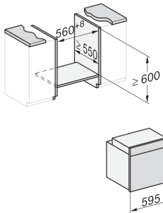
Installation H7000 XL underframe, installation drawings
