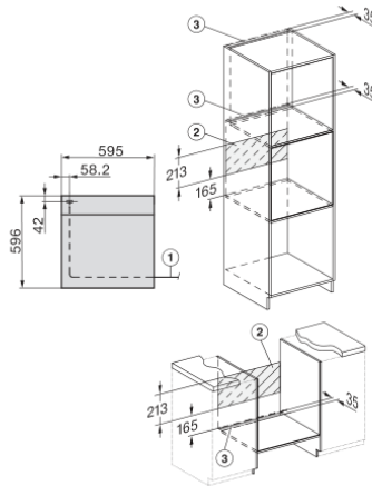
installation H7000 XL, installation drawing, GB, AU
