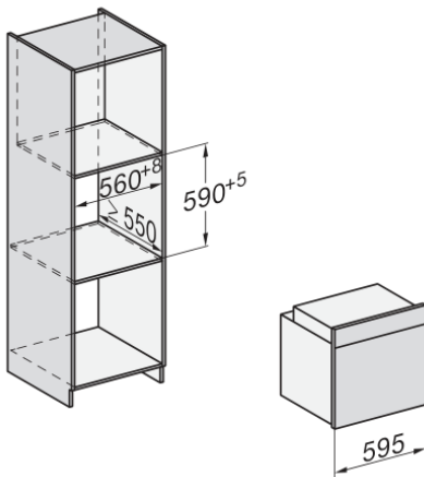
built-in H7000 XL, installation drawing
