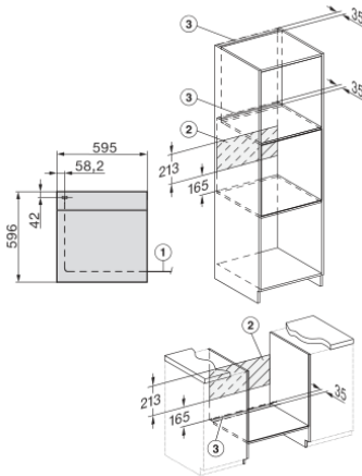
installation H7000 XL, installation drawing
