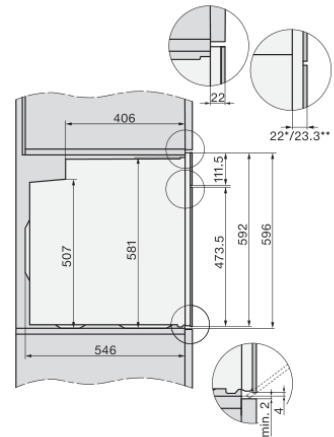
side view H7000 XL, installation drawings, GB,
