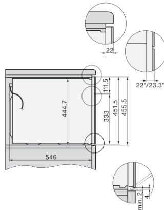
Installation H7000BM, installation drawings, GB, AUS 1) Mains connection cable, L=2000 mm, 2) No connection in this area, 3) Lüftungsausschnitt min. 150 cm²
