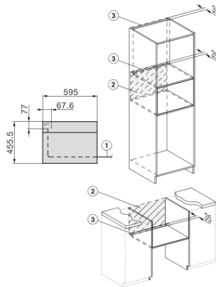
Installation H7000BM, installation drawings, GB, AUS 1) Mains connection cable, L=2000 mm, 2) No connection in this area, 3) Lüftungsausschnitt min. 150 cm²
