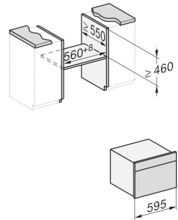
built-in H7000 BM build-under, installation drawing
