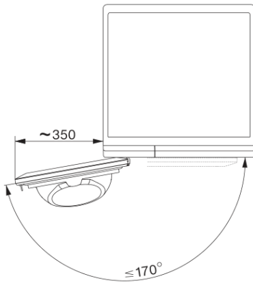
T1 installation drawing, slanted fascia or straight fascia, measures in mm
