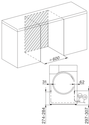
T1 Skizze, 5 Grad Blende, Maße in mm
