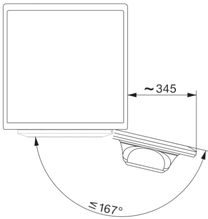
WT1 8/5 kg, installation drawing, slanted facia or straight facia, measures in mm
