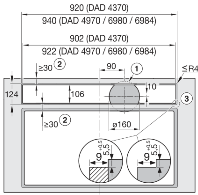
DAD4370, DAD4970, DAD6980, flush, Installation drawings
