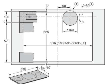
DAD4970, DAD6980, surface mounted installation, common cutout, Installation drawings
