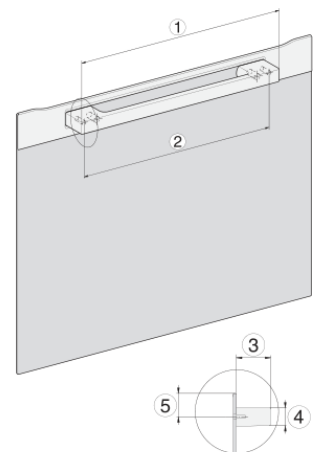
H7000 handle, installation drawing
