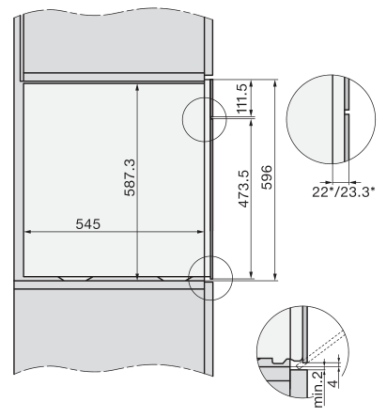
screw joint DGC XXL, installation drawing
