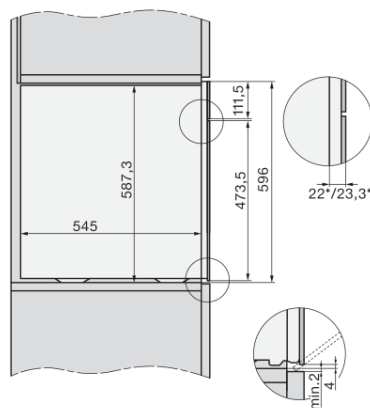
built-in DGC XXL build-under, installation drawing Worktop overhang ≤ 29 mm
