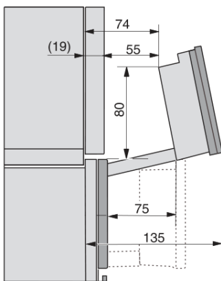
built-in DGC XXL, installation drawing
