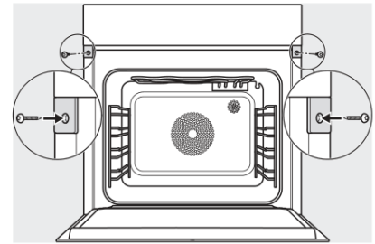
Installation_DGC_XXL_ESW7x10_EVS7010 installation drawings
