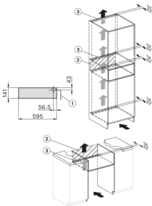
built-in ESW7x10 EVS7010, installation drawing
