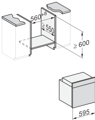
installation H7000 XL, installation drawing
