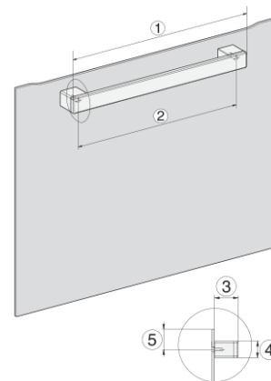
built-in H7000 XL, installation drawing
