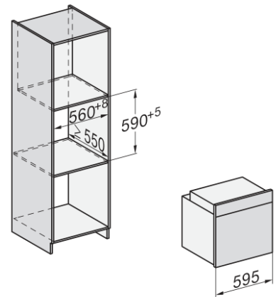
built-in H7000 XL, installation drawing
