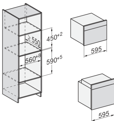
built-in H7000 BM build-under, installation drawings If the oven is to be installed under a hob, follow the instructions for installing the hob and the height of the hob.
