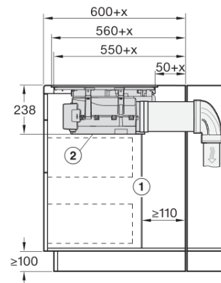
KMDA7272-1FL/FR, KMDA7473-1FL/FR, KMDA7473-1FL MattFinish, KMDA7676-1FL, KMDA7876-1FL – Operating options
