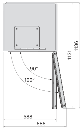
KWTUS7196E, KWTUS7096E, Built-under, top view
