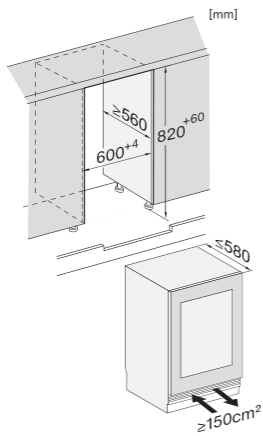
KWTUS7054F, KWTUS7055F, KWTUS7074F, KWTUS7096E, Built-under, niche dimensions
