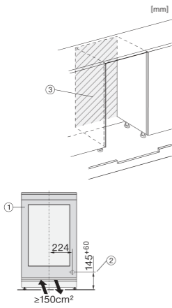
KWTUS7054F, KWTUS7055F, KWTUS7074F, KWTUS7096E, Built-under, niche dimensions
