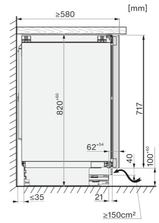
KWTUS7096E, Built-under, side view
