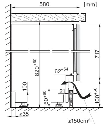
KWTUS7096E, Built-under, side view
