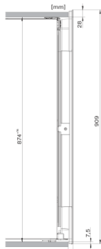
KWT6422iG, KWT6422iG-1, Installation draw, side view
