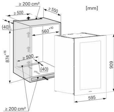
KWT6422iG, KWT6422iG-1, Installation draw
