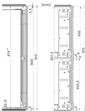
KWT6422iG, KWT6422iG-1, Installation draw, side view
