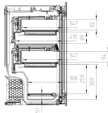
KWT6422iG, KWT6422iG-1, Interior dimensions (Installation drawings)
