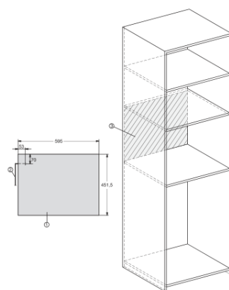
M7140TC, M724xTC, installation drawing
