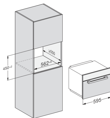
M7140TC, M724xTC, installation drawing 22 mm – glass, 23.3 mm – stainless steel
