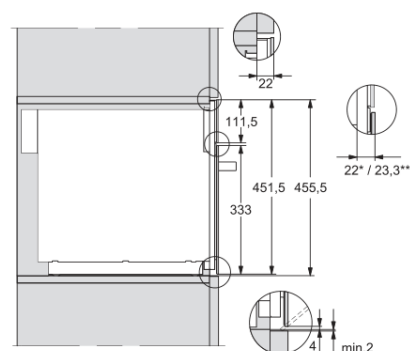
M7140TC, M724xTC, installation drawing 22 mm – glass, 23.3 mm – stainless steel
