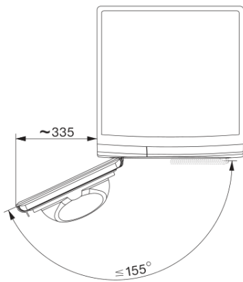
T1 installation drawing, facia 5 degree, measures in mm
