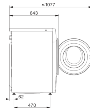
W1 drawing, facia 5 degree, measures in mm
